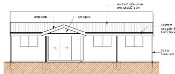
ELEVATION 1 SCALE 1:100
