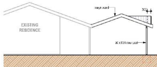
ELEVATION 2 SCALE 1:100
